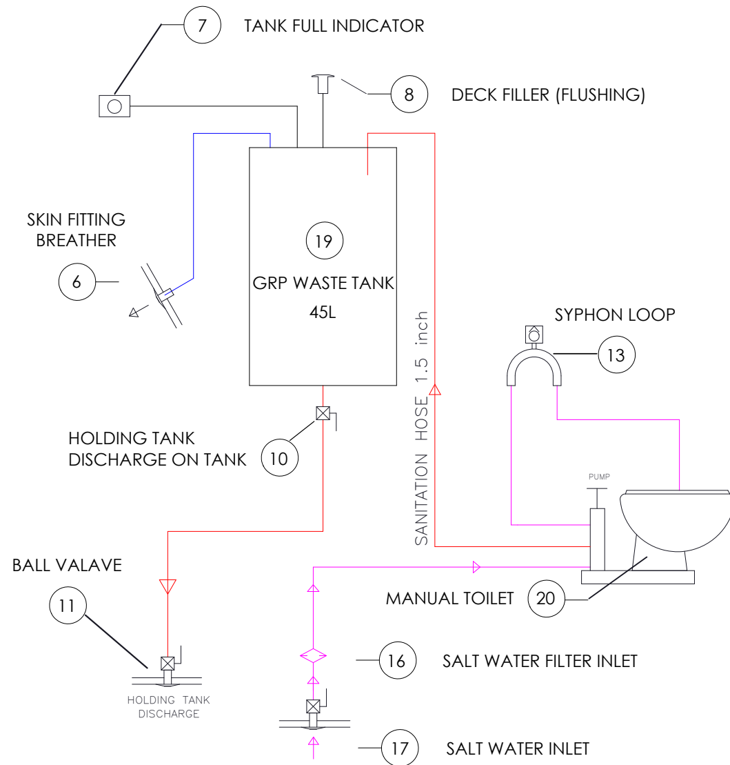
MANUAL TOILET SCHEMATIC
