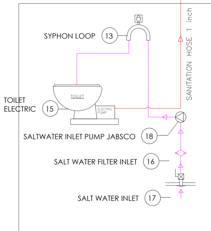
PORT AFT HEADS TOILET SCHEMATIC SHOWN WITH ELECTRIC TOILET OPTION
