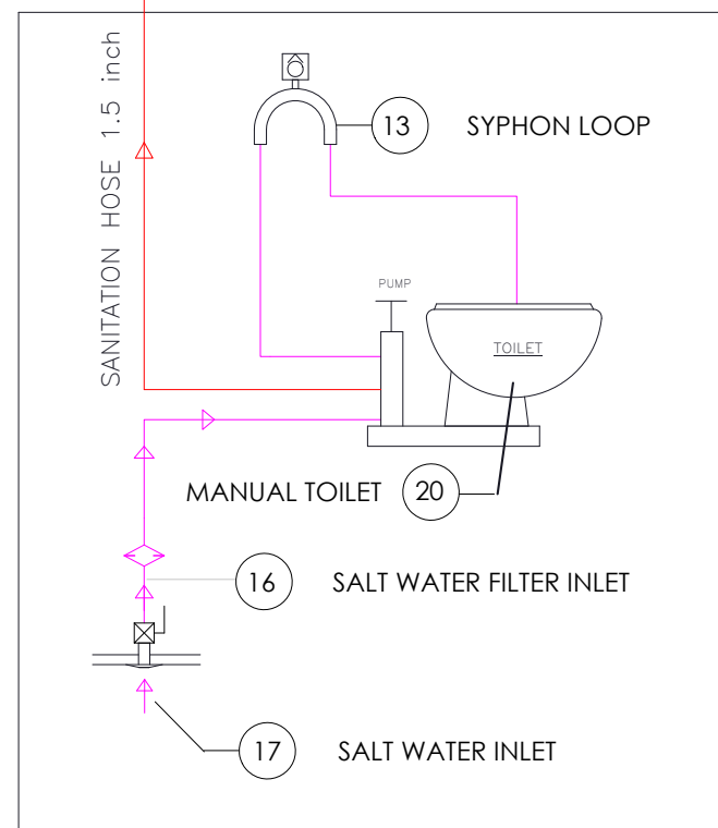
PORT FWD HEADSTOILET SCHEMATIC SHOWN WITH STANDART MANUAL TOILET
